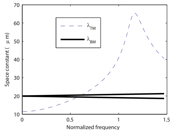
FIG. 5. (Color online) Space constants characteristic of BM longitudinal coupling ( \lambda_{BM} ) and TM longitudinal coupling ( \lambda_{TM} ) as a function of the frequency (normalized to the CF). For BM longitudinal coupling there are two space constants because Eq. (5) is quadratic in k_{bm} (Ref. 2). At low frequencies the space constants for the BM and the TM are similar (about 20 \mu\text{m} for the BM and 12 \mu\text{m} for the TM). But close to CF, the space constants characteristic of TM longitudinal coupling are more than three times as high as the space constant characteristic of BM longitudinal coupling.
