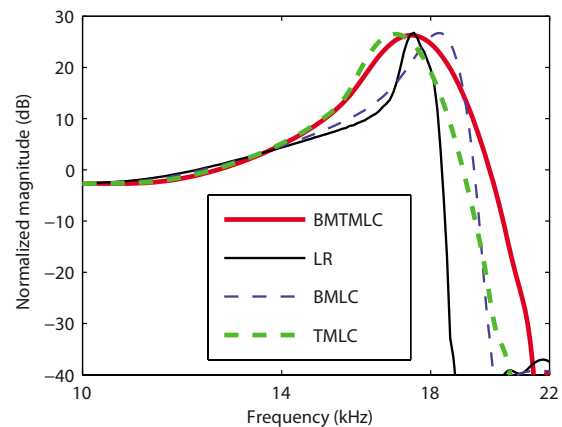
FIG. 2. (Color online) Model predictions for the BM gain in the active case (80% activity). As in Ref. 19, the gain is normalized to the maximum passive model gain. Thin solid line: Active LR model response. Thick dashed line: Active TM-LC model response. Thin dashed line: Active BM-LC model response. Thick solid line: Active TMBM-LC model response. The values for \epsilon_3(x) for the different models are given in Table III. The four models are capable of predicting realistic maximum gains but at these activity levels the Q_{10 \text{ dB}} for the LR and BM-LC models are always much higher than that predicted by the TM-LC and TMBM-LC models.
